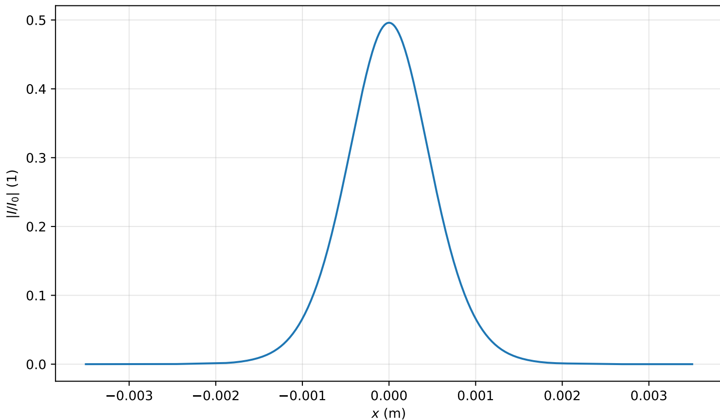
Intensity profile I(x, y = 0, z = 3.344m)/I_0 , P_{in}=0.5P_{cr} , artificial time
